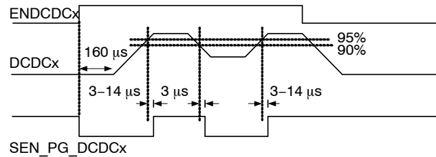
Figure 61. DCDCx Channel Internal Power Good Signal
