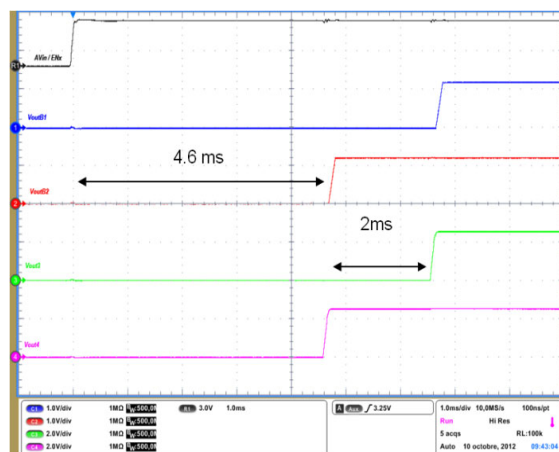
Figure 48. NCP6922CB Power-up Sequence All Enable pins high
