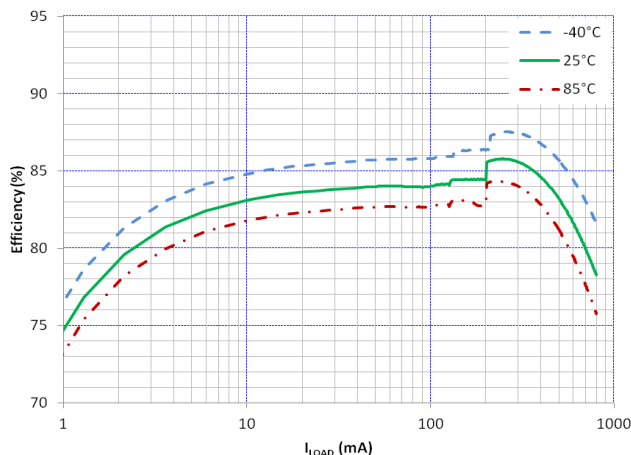
Figure 14. Efficiency vs I_{LOAD} and V_{IN} DCDC2 – V_{OUT} = 3.30\text{ V} , SPM3012 Inductor
