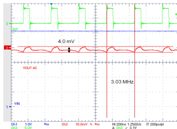
Figure 46. Ripple voltage in PWM mode DCDC2, V_{OUT} = 1.20\text{ V} , I_{OUT}=200\text{mA}
