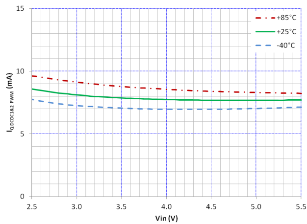
Figure 31. I_{Q\ PWM} vs VIN and Temperature
