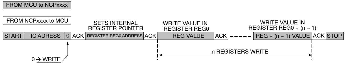
Figure 72. Write In n Registers
