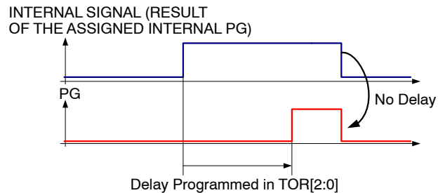
Figure 66. PG Delay
