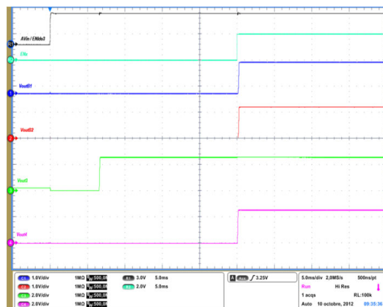
Figure 50. NCP6922CB power-up sequence All ENx after the power up sequence
