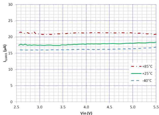
Figure 29. I_{Q\ LDO3} vs VIN and Temperature
