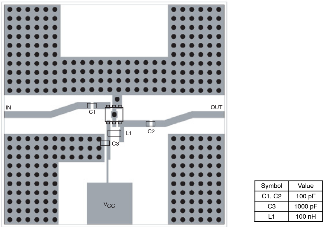
Figure 2. Evaluation Board
