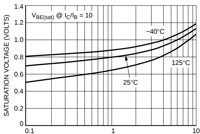
Figure 8. D45VH10 ON-Voltage
