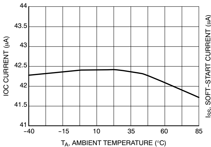
Figure 8. IOC Current vs Ambient Temperature
