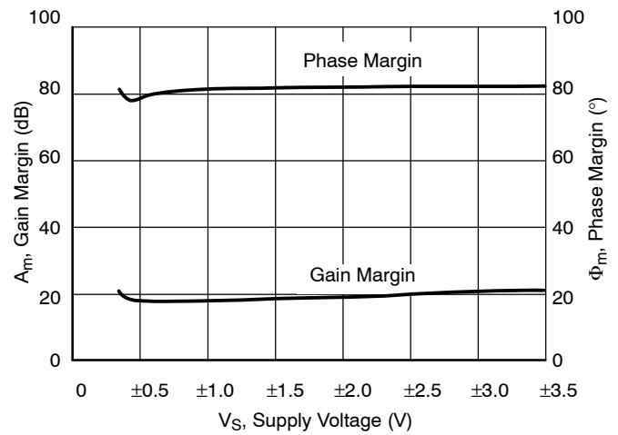
Figure 25. Gain and Phase Margin versus Supply Voltage
