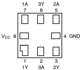
Figure 4. MicroPak (Top Through View)
