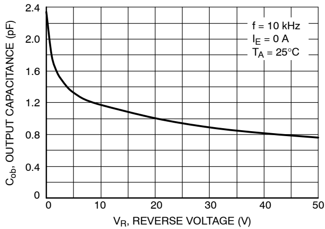
Figure 10. Output Capacitance
