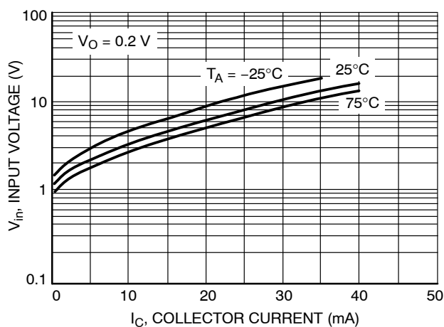
Figure 7. Input Voltage vs. Output Current
