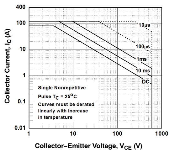
Figure 11. SOA Characteristics
