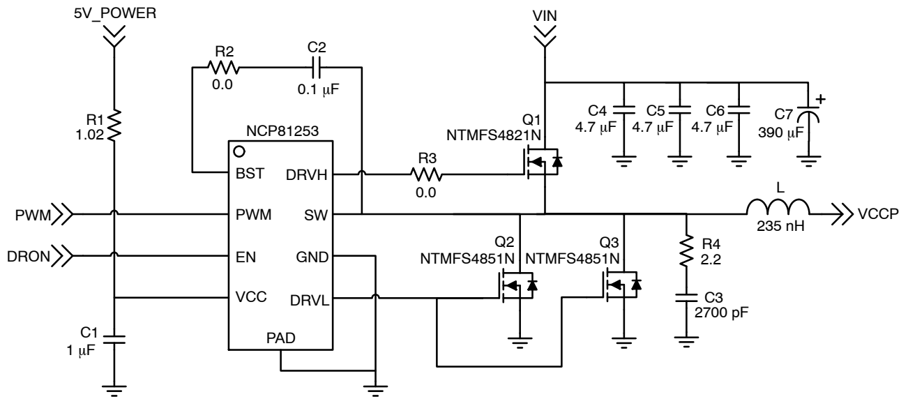
Figure 14. Application Circuit
