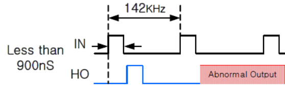
Figure 5. Abnormal Output Waveform with Pulse Width
