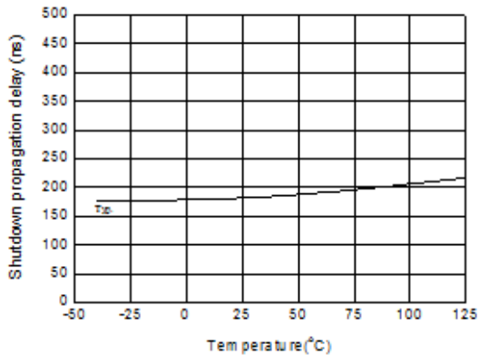
Figure 60. Shutdown Propagation Delay vs. Temperature
