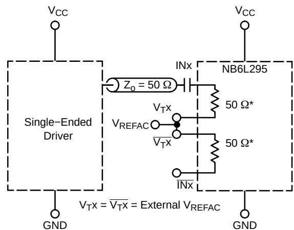
Figure 20. Capacitor-Coupled Single-Ended Interface (VTx/VTx- Connected to External VREFAC; VREFAC Bypassed to Ground with 0.1 μF Capacitor)
