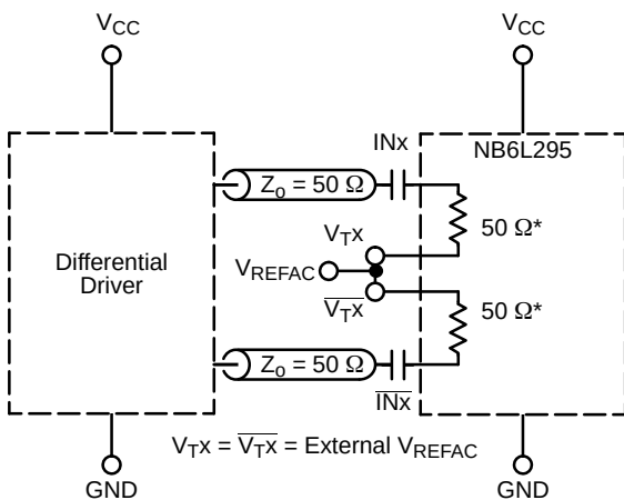
Figure 19. Capacitor-Coupled Differential Interface (VTx/VTx- Connected to VREFAC; VREFAC Bypassed to Ground with 0.1 μF Capacitor)
