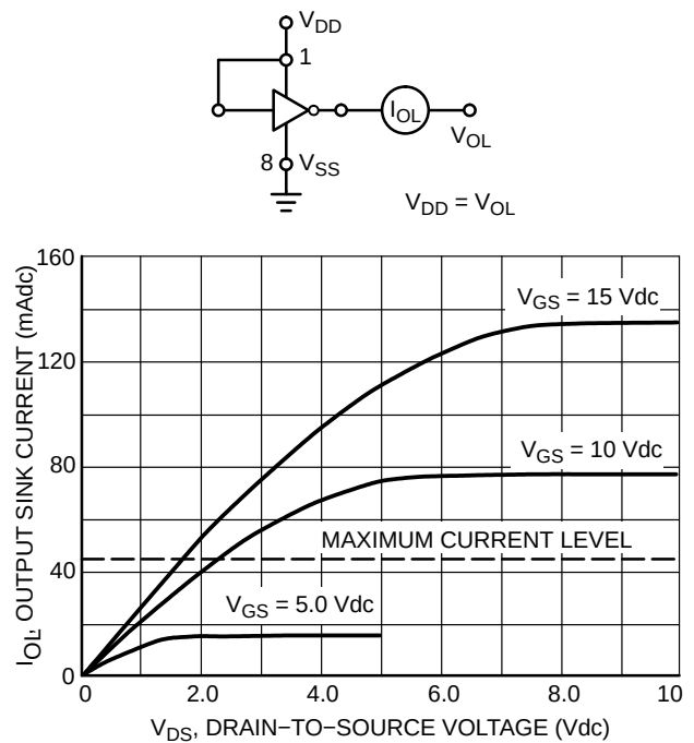
Figure 6. Typical Output Sink Characteristics
