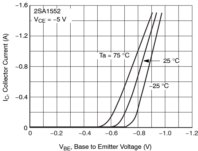
Figure 6. I_C - V_{BE}
