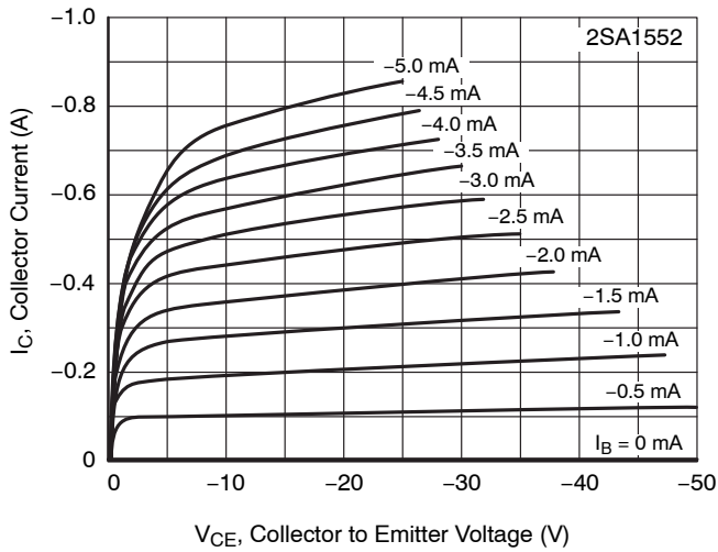
Figure 4. I_C - V_{CE}
