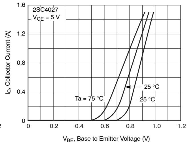
Figure 7. I_C - V_{BE}
