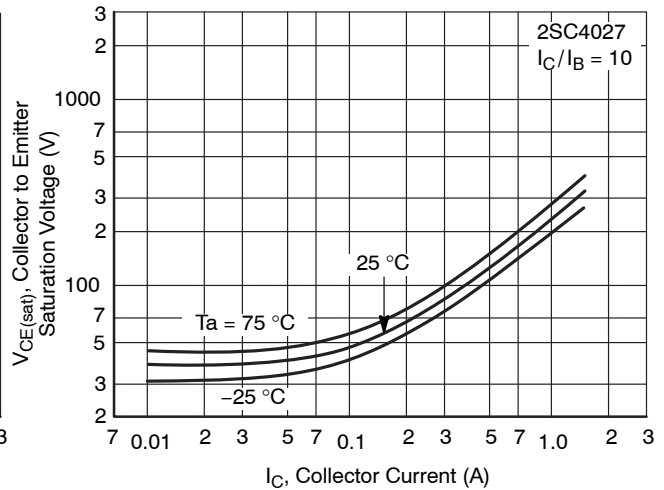
Figure 13. V_{CE(sat)} - I_C
