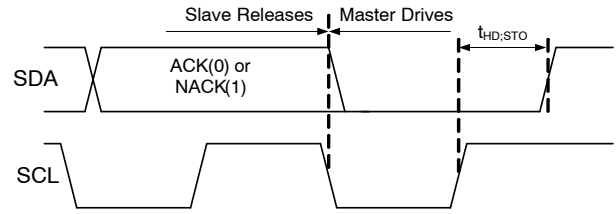
Figure 39. Stop Bit
