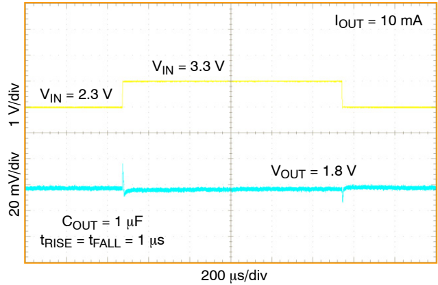
Figure 54. Line Transient 2.3 V – 3.3 V NCP752A/B, V OUT = 1.8 V
