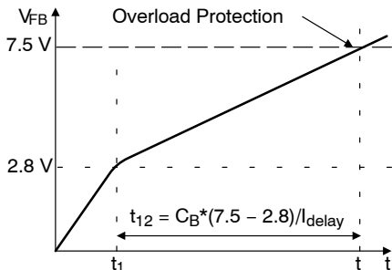
Figure 34. Overload Protection
