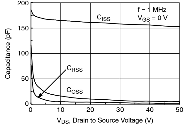
Figure 8. Capacitance Characteristics
