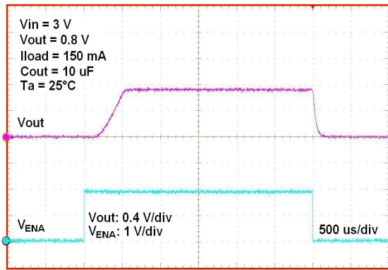
Figure 17. Enable Operation
