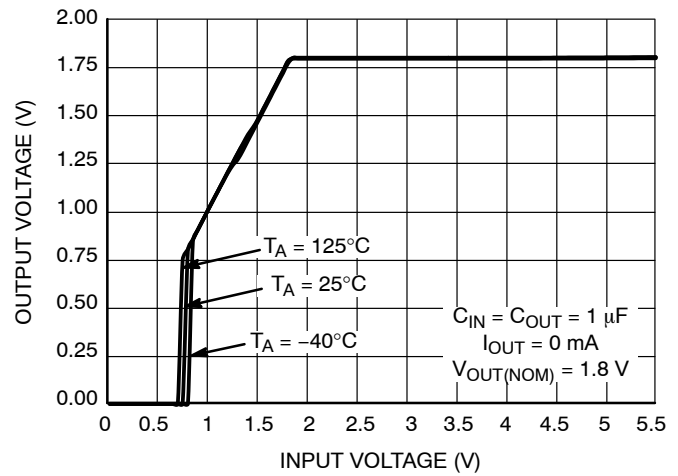
Figure 16. Output Voltage vs. Input Voltage V_{OUT} = 1.8\ \text{V}
