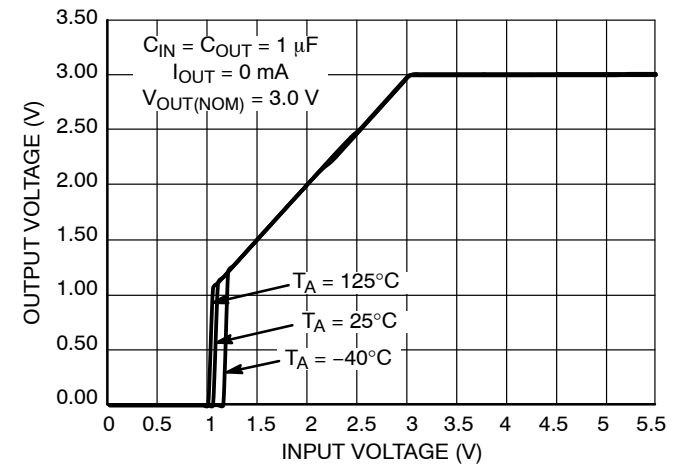
Figure 18. Output Voltage vs. Input Voltage V_{OUT} = 3.0\ \text{V}
