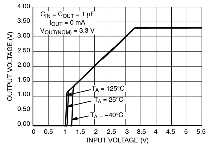
Figure 20. Output Voltage vs. Input Voltage V_{OUT} = 3.3\ \text{V}
