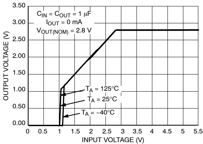
Figure 17. Output Voltage vs. Input Voltage V_{OUT} = 2.8\ \text{V}
