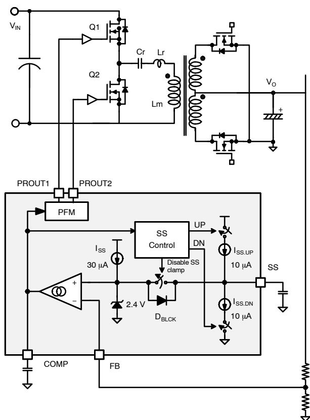
Figure 68. Schematic of Closed Loop Soft-Star
