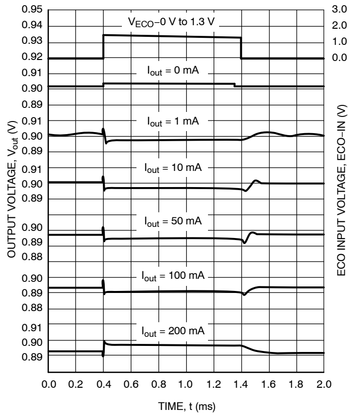
Figure 31. Output Voltage at Mode Alternative Point ( C_{in} = 1.0\text{ }\mu\text{F} , C_{out} = 2.2\text{ }\mu\text{F} , 8.0\text{ V} , V_{out} = 0.9\text{ V} )
