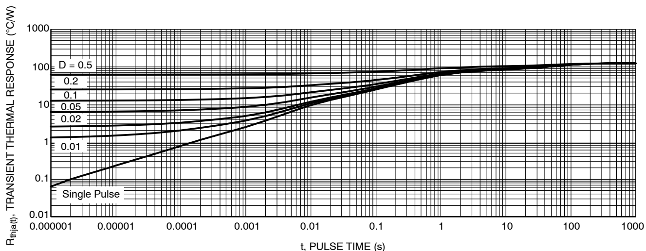
Figure 15. Thermal Response
