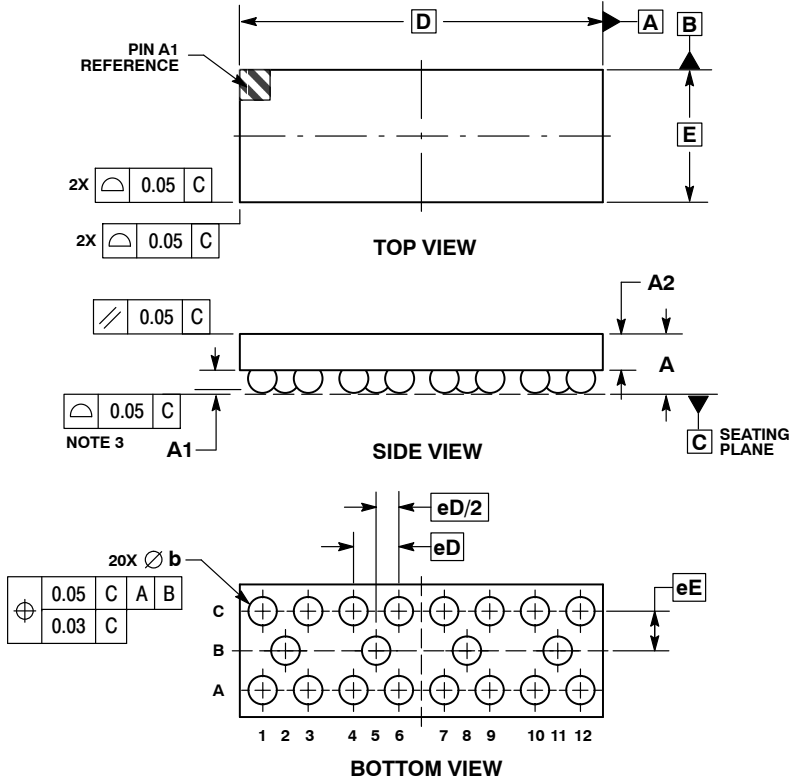
WLCSP20, 4.00x1.46 CASE 567BZ ISSUE O
