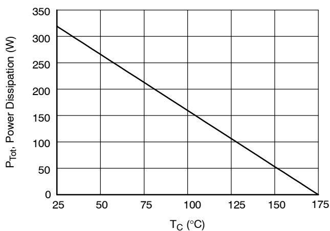
Figure 4. Power Dissipation
