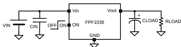
Figure 28. Device Setup
