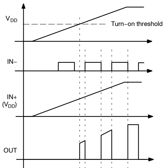
Figure 53. Inverting Startup Waveforms
