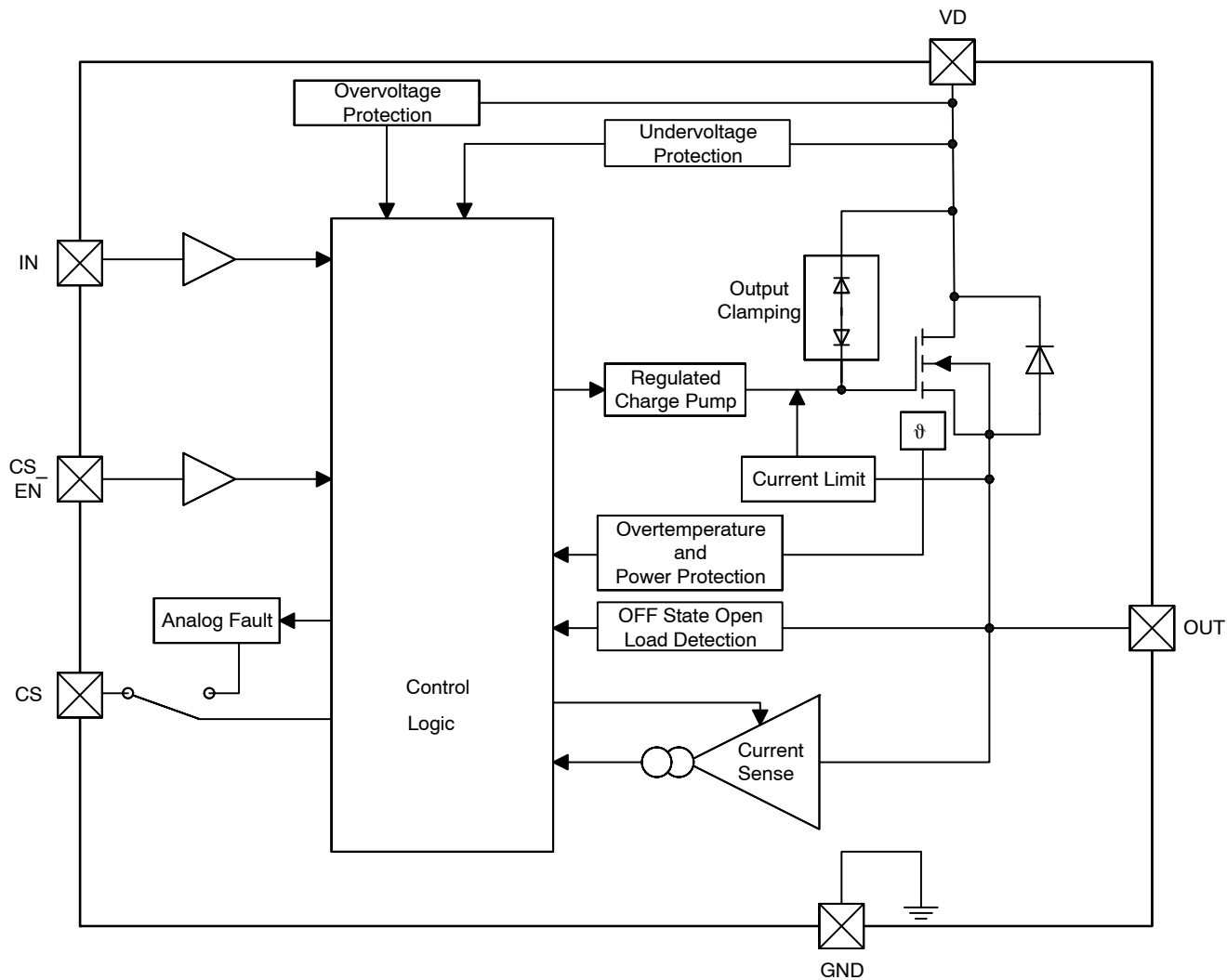
Figure 1. Block Diagram
