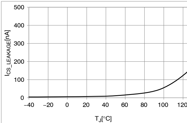
Figure 23. CS Input Leakage V_{CS} = 200\text{ V}
