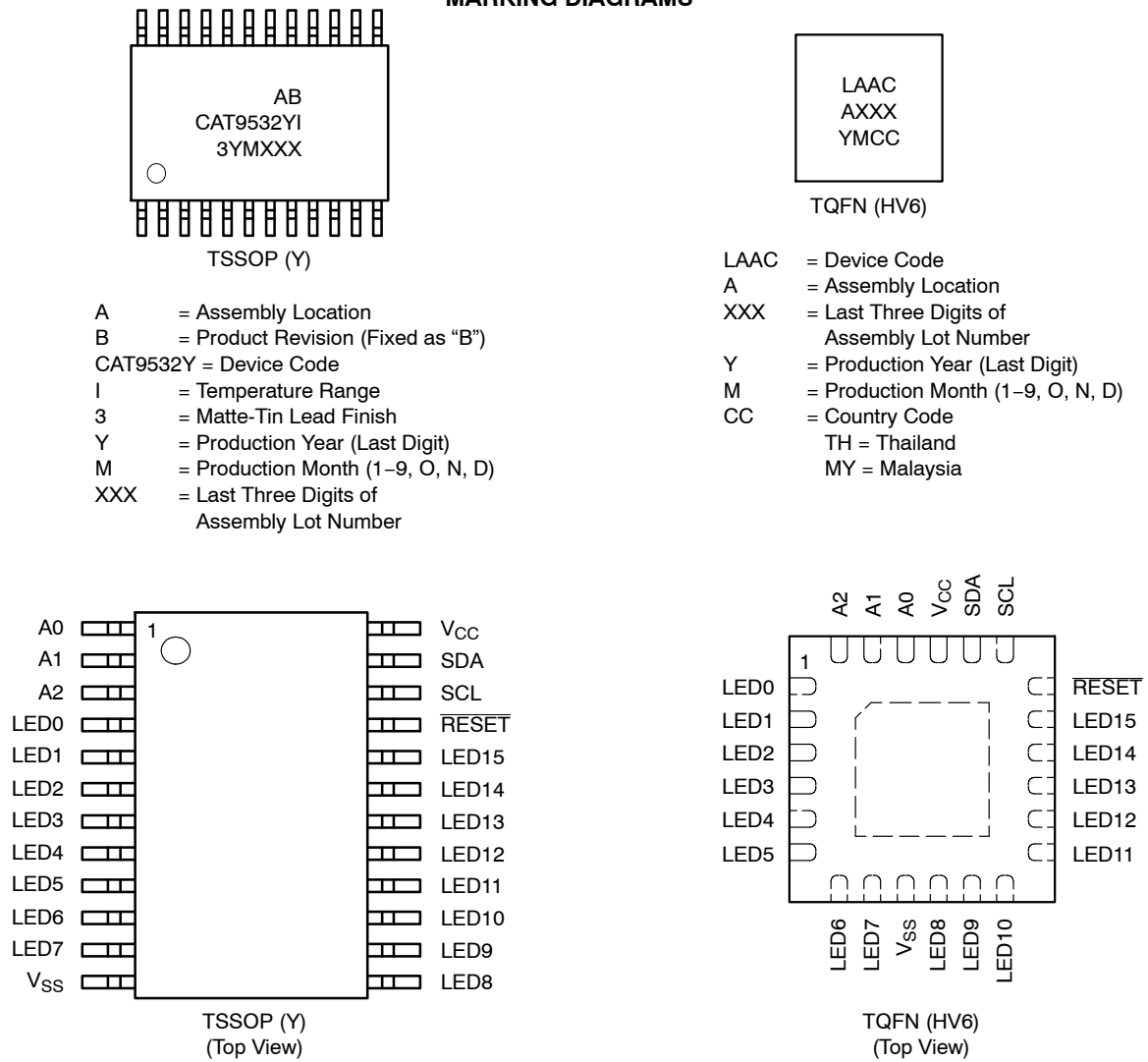
Figure 1. Pin Configurations
