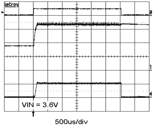
Figure 11. Power-up Transient (2 LEDs at 200 mA)
