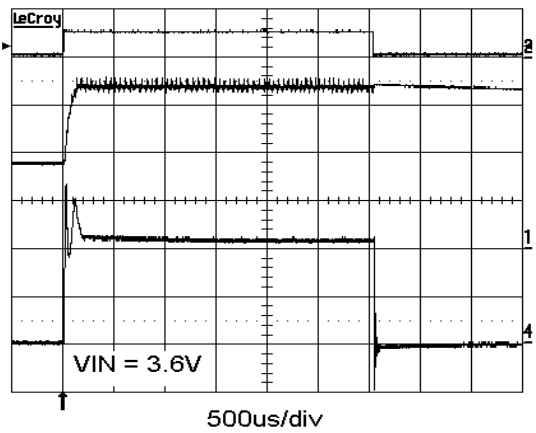
Figure 9. Power-up Transient (2 LEDs at 200 mA)
