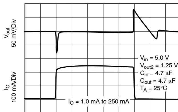
Figure 18. Load Transient Response for V_{out2}
