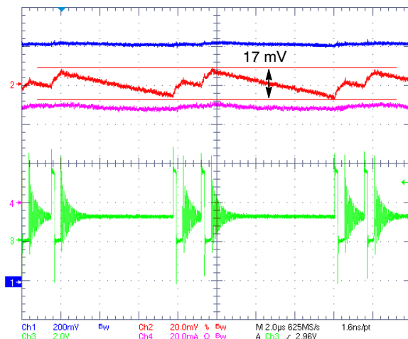
Figure 25. PFM Ripple
