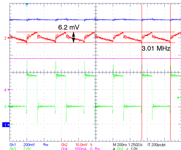
Figure 24. PWM Ripple
