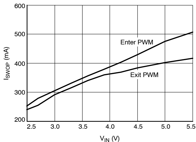
Figure 23. Switchover Point V_{\text{OUT}} = 1.39375\text{ V}
