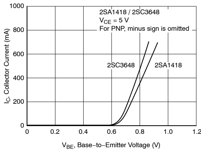
Figure 6. I_C - V_{BE}
