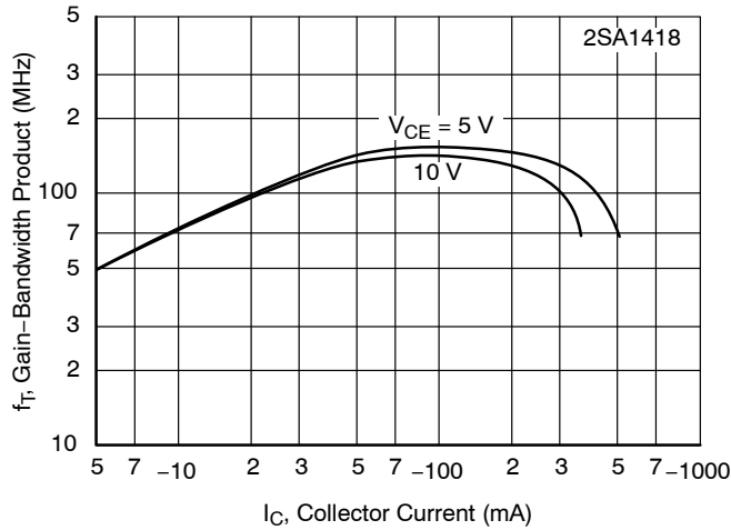
Figure 10. f_T - I_C
