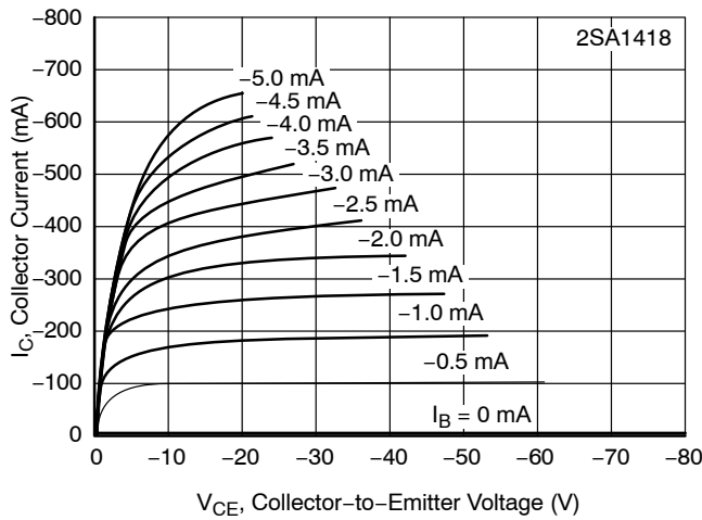
Figure 4. I_C - V_{CE}
