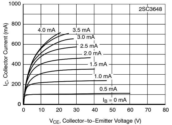
Figure 5. I_C - V_{CE}
