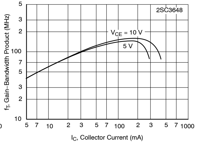
Figure 11. f_T - I_C
