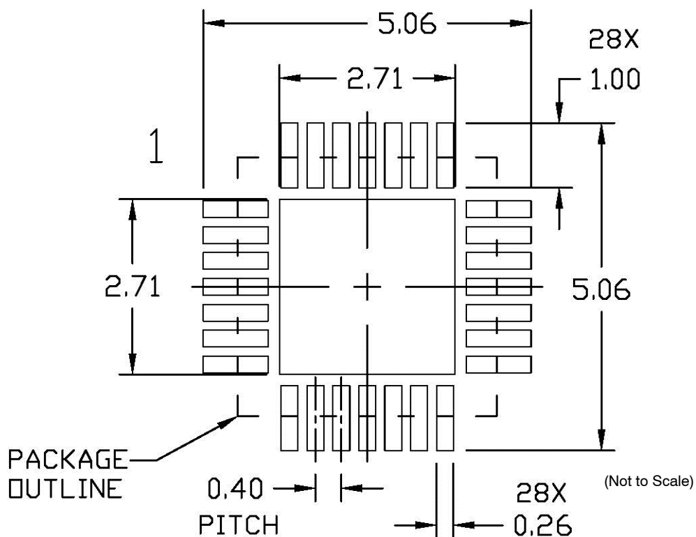
Figure 10. Alternative Extended Soldering Footprint
