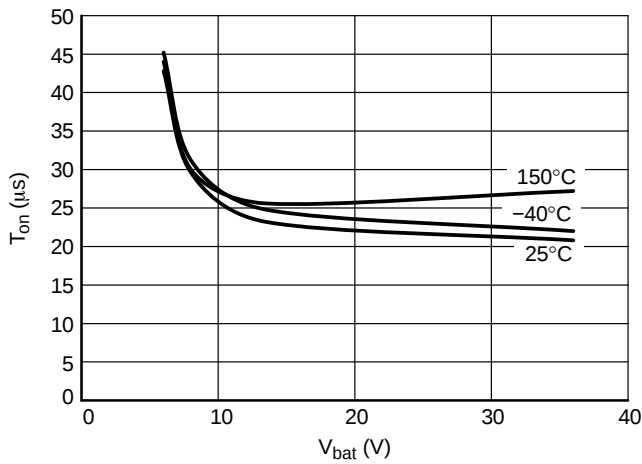
Figure 15. Turn On Delay Time vs. V_{bat} and Temperature
