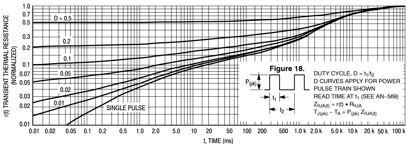
Figure 17. Thermal Response
