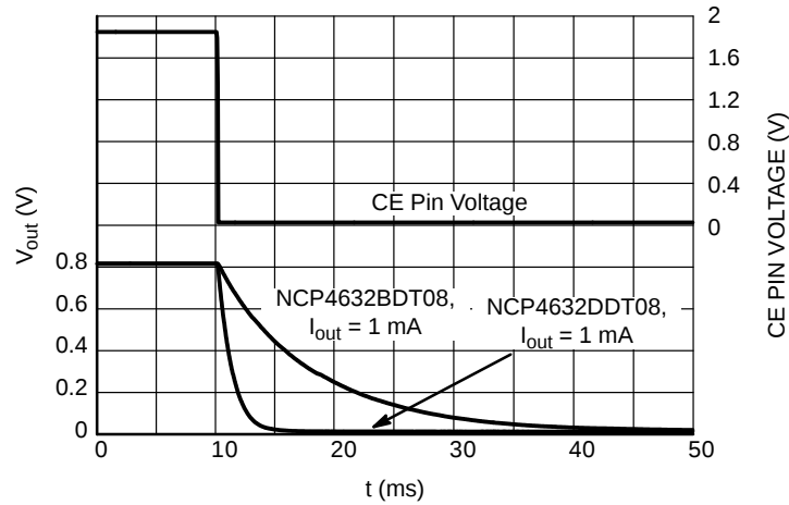
Figure 33. Turn Off with CE pin at NCP4632BDT08, NCP4632DDT08, I_{out} = 1 \text{ mA}
