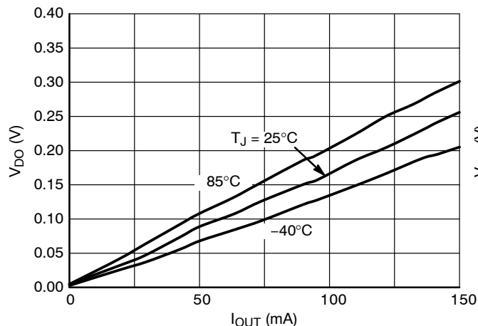
Figure 6. Dropout Voltage vs. Output Current 3.3 V Version
