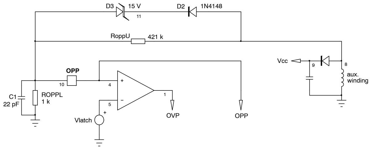
Figure 38. A Zener diode in series with a diode helps to improve the noise immunity of the system.
