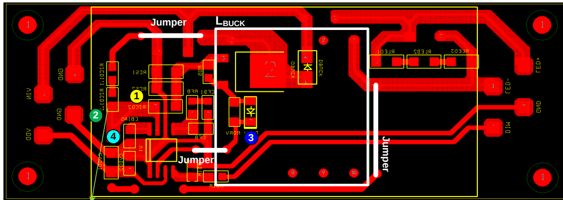
Figure 16. Layout Guidance
