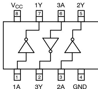
Figure 2. Connection Diagram
