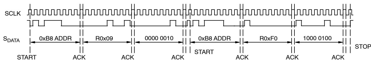
Figure 12. Timing Diagram Showing a Byte-wise Write to R0x09 with Value 0x0284
