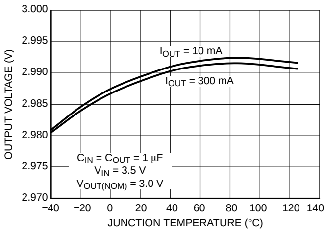
Figure 4. Output Voltage vs. Temperature V_{OUT} = 3.0 \text{ V}
