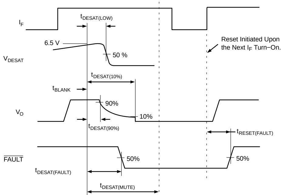
Figure 4. Definitions for DESAT, V_O and \overline{\text{FAULT}} Timing Waveforms
