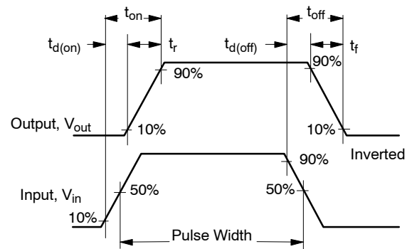
Figure 12. Switching Waveforms
