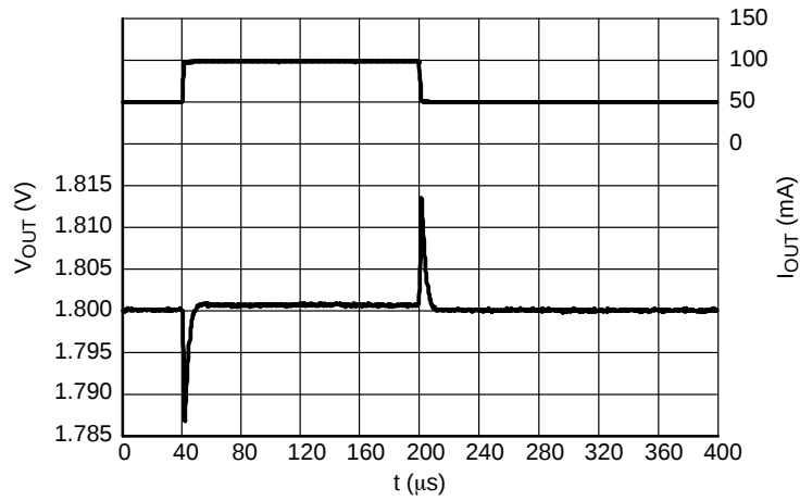
Figure 44. Load Transients, 1.8 V Version, I_{OUT} = 50 - 100 \text{ mA} , t_R = t_F = 0.5 \mu s , V_{IN} = 2.8 \text{ V}
