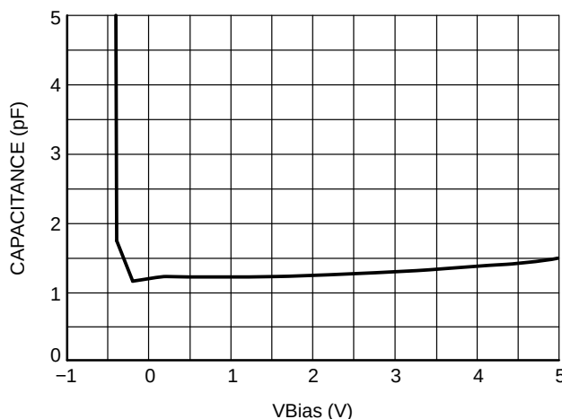
Figure 6. CV Characteristic Curve
