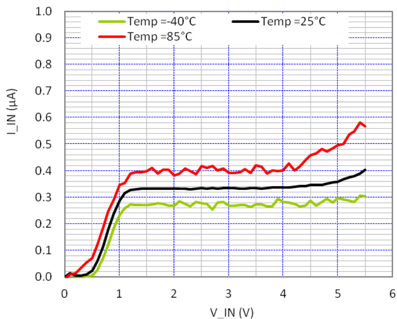
Figure 4. Standby Current ( \mu A ) versus V_{in} (V)
