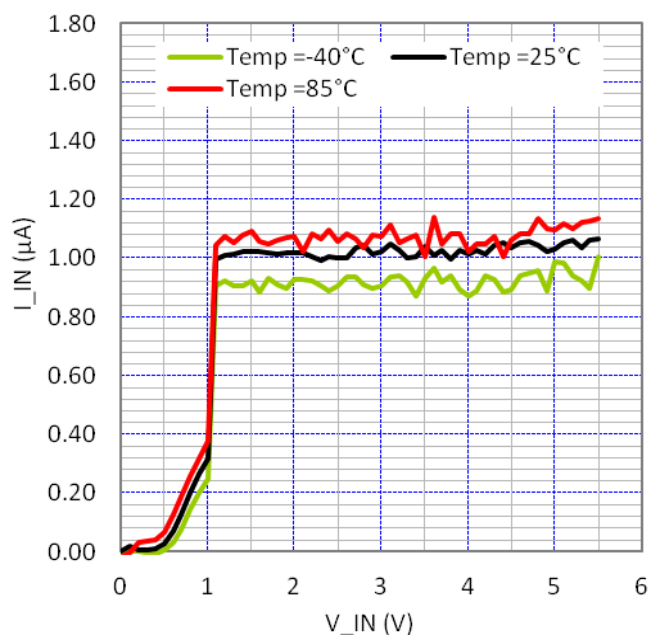
Figure 5. Quiescent Current ( \mu A ) versus V_{in} (V)
