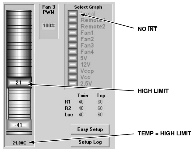
Figure 30. Temperature = High Limit: No INT
