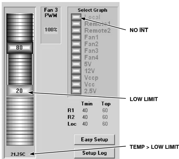
Figure 28. Temperature &gt; Low Limit: No INT
