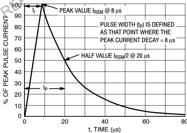
Figure 11. 8 X 20 \mu s Pulse Waveform
